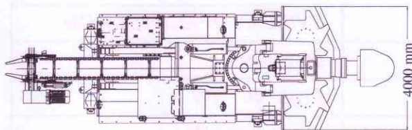
Mk 4 excavation profile
