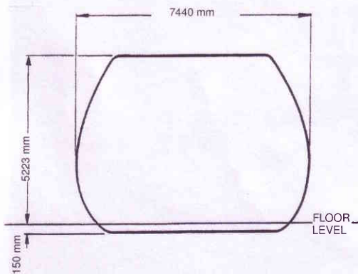
Mk 4 excavation profile
